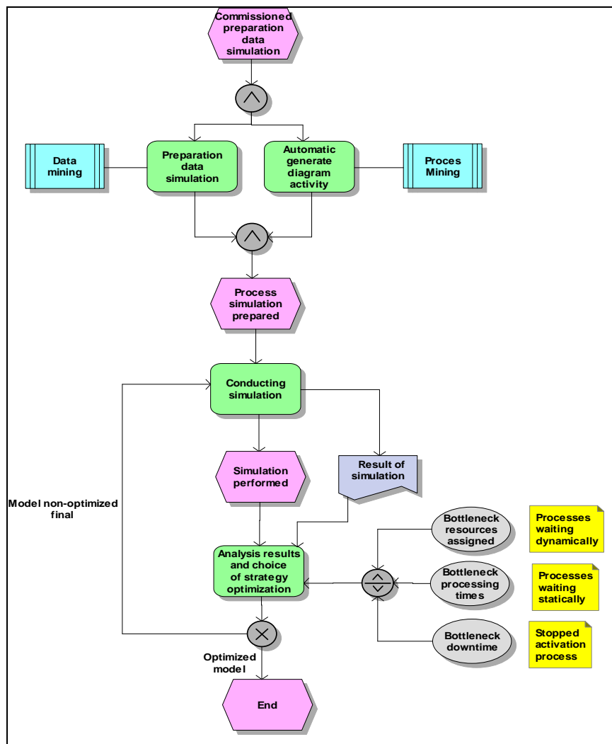
Figure 4: Developed method of procedure to carry out whole study
